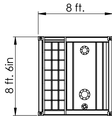
ELEVATION SIDE
