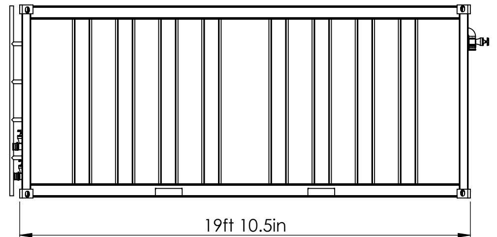
ELEVATION FRONT
